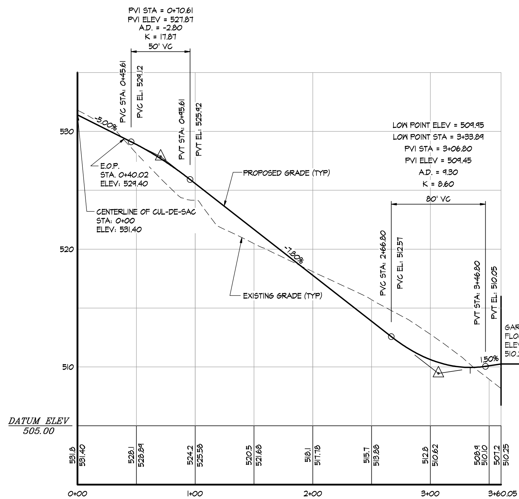
D DRIVWAY PROFILE: LOT #3 SCALE: HORIZ. 1"=50', VERT. 1"=5'
