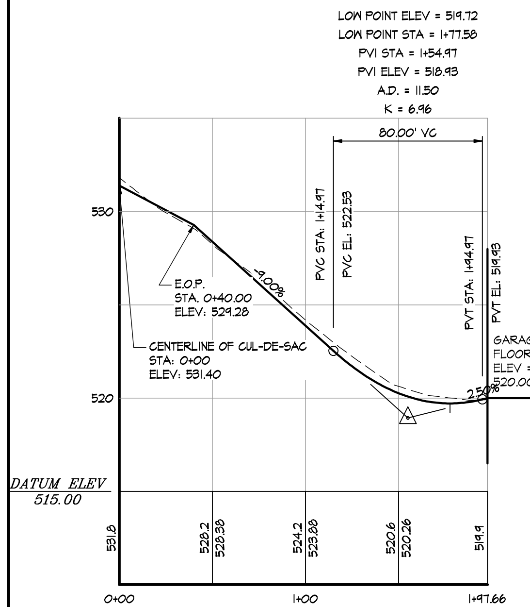
C DRIVWAY PROFILE: LOT #2 SCALE: HORIZ. 1"=50', VERT. 1"=5'
