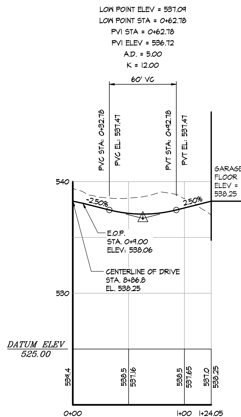
B DRIVWAY PROFILE: LOT #1 SCALE: HORIZ. 1"=50', VERT. 1"=5'
