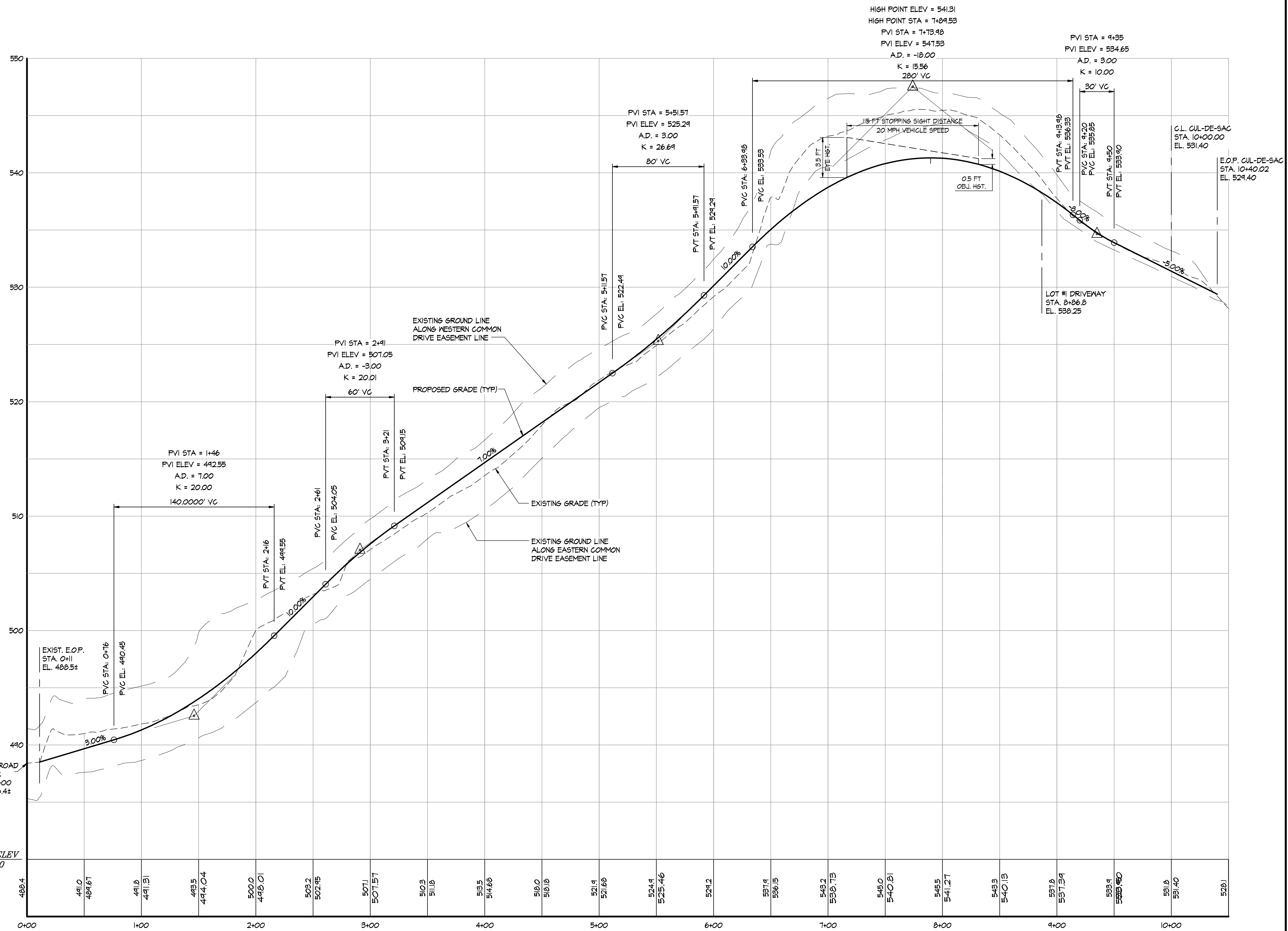
A ACCESS ROAD PROFILE SCALE: HORIZ. 1"=50', VERT. 1"=5'
