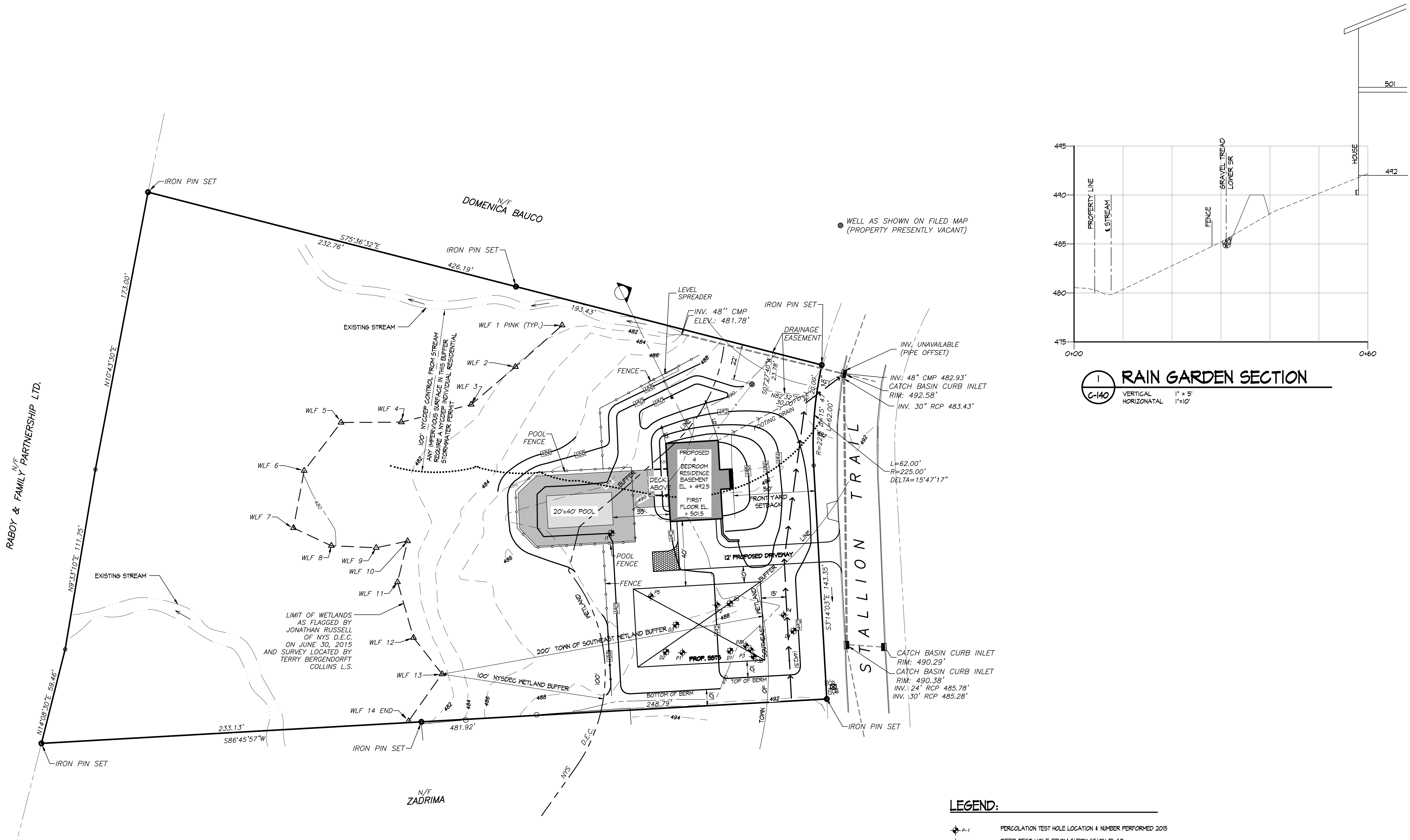
GRADING PLAN GRAPHIC SCALE 1 INCH = 30 FEET
